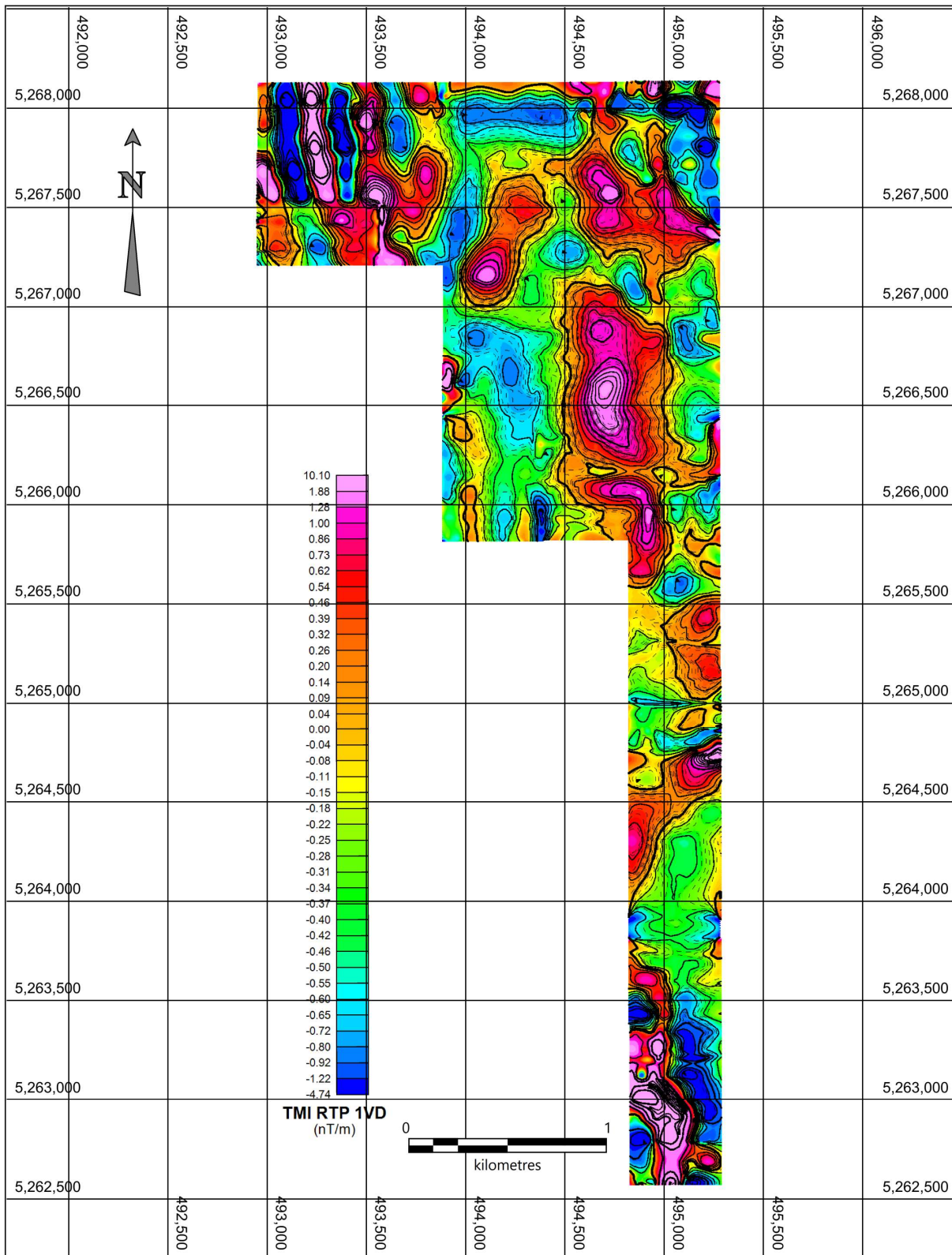
Figure 6. Initial Interpretation (1st Vertical Derivative) of Drone Magnetics
